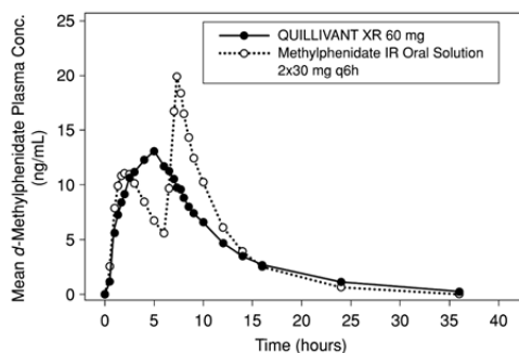
Figure 2. Mean d -Methylphenidate Plasma Concentration-Time Profiles
